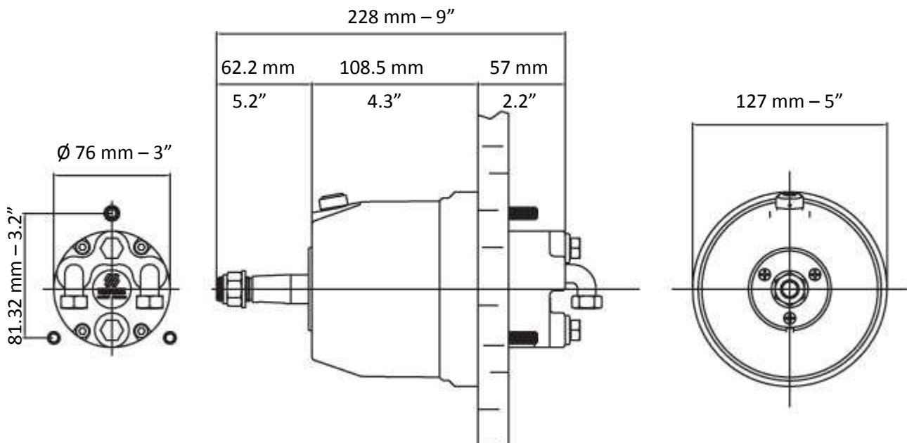
DIMENSIONS UP20F
