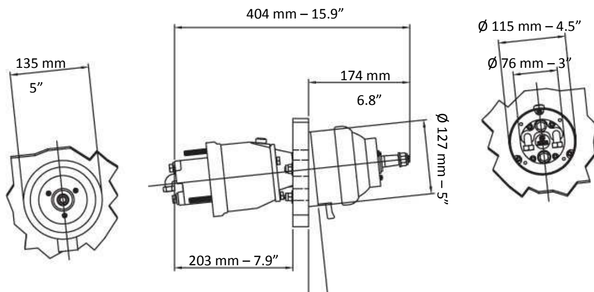
DIMENSIONS UP20T
