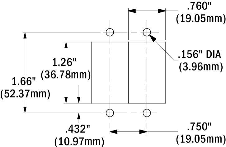
PANEL CUTOUT DETAIL
