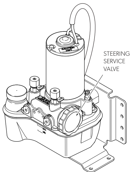
Figure 11-7. Hydraulic pump and reservoir.
