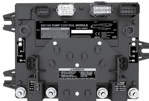
Figure 11-6. Pump control module.
