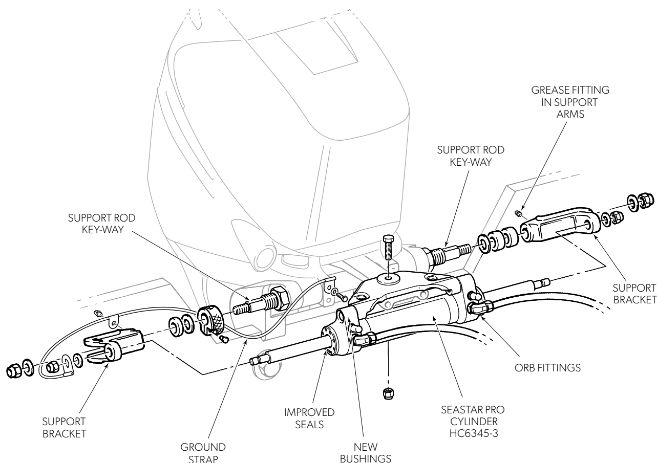
Figure 3-18. Cylinder part # HC6345-3 shown.
