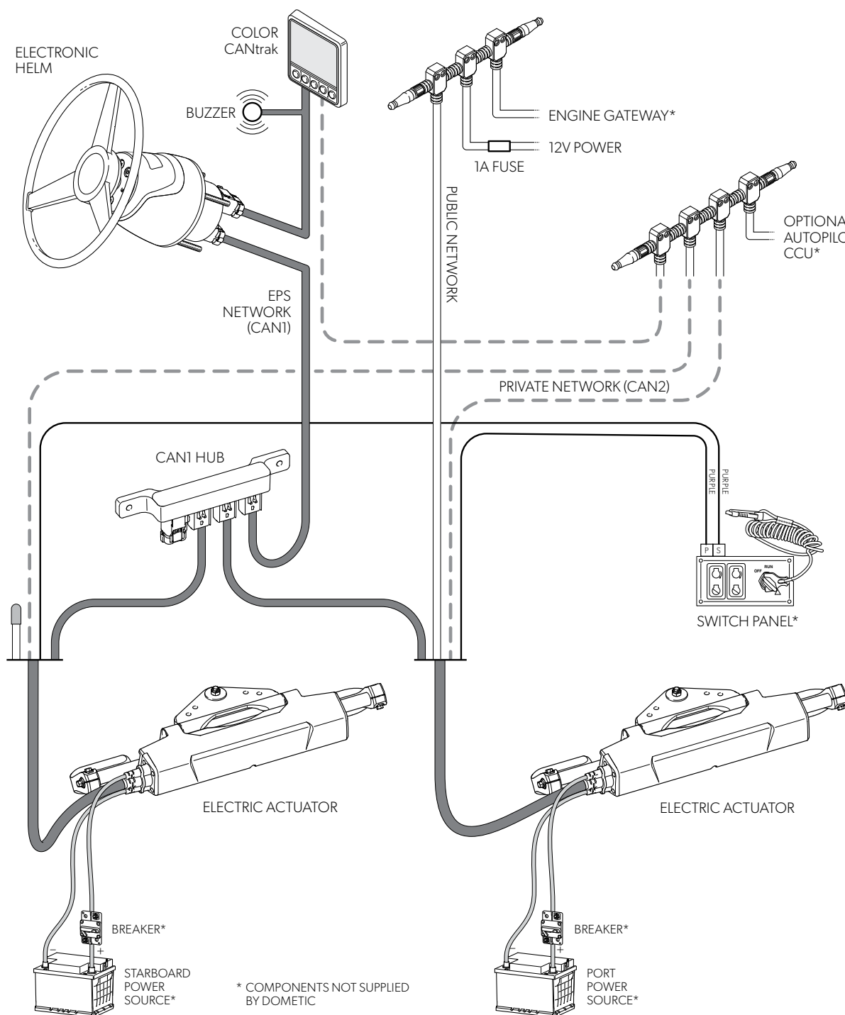
Figure 11-13. Optimus EPS electric actuator system diagram, single station, twin engine.
