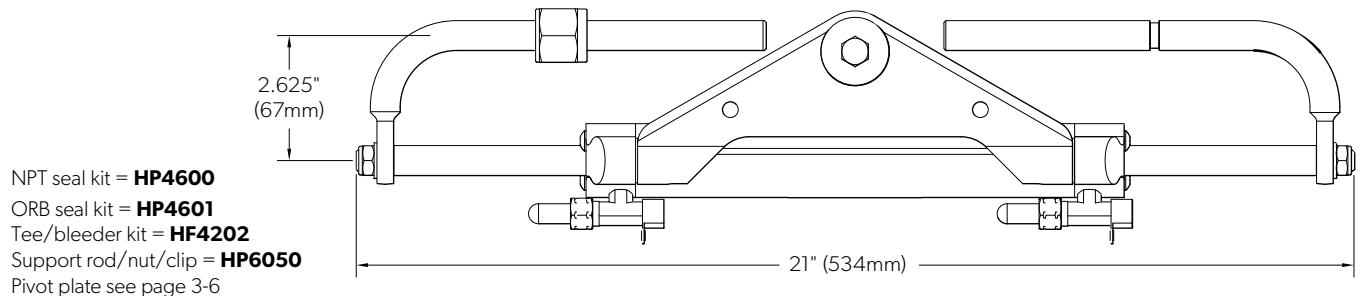
Figure 3-6. BayStar cylinder part # HC4645-3 / 47-3 / 48-3 / 58-3.
