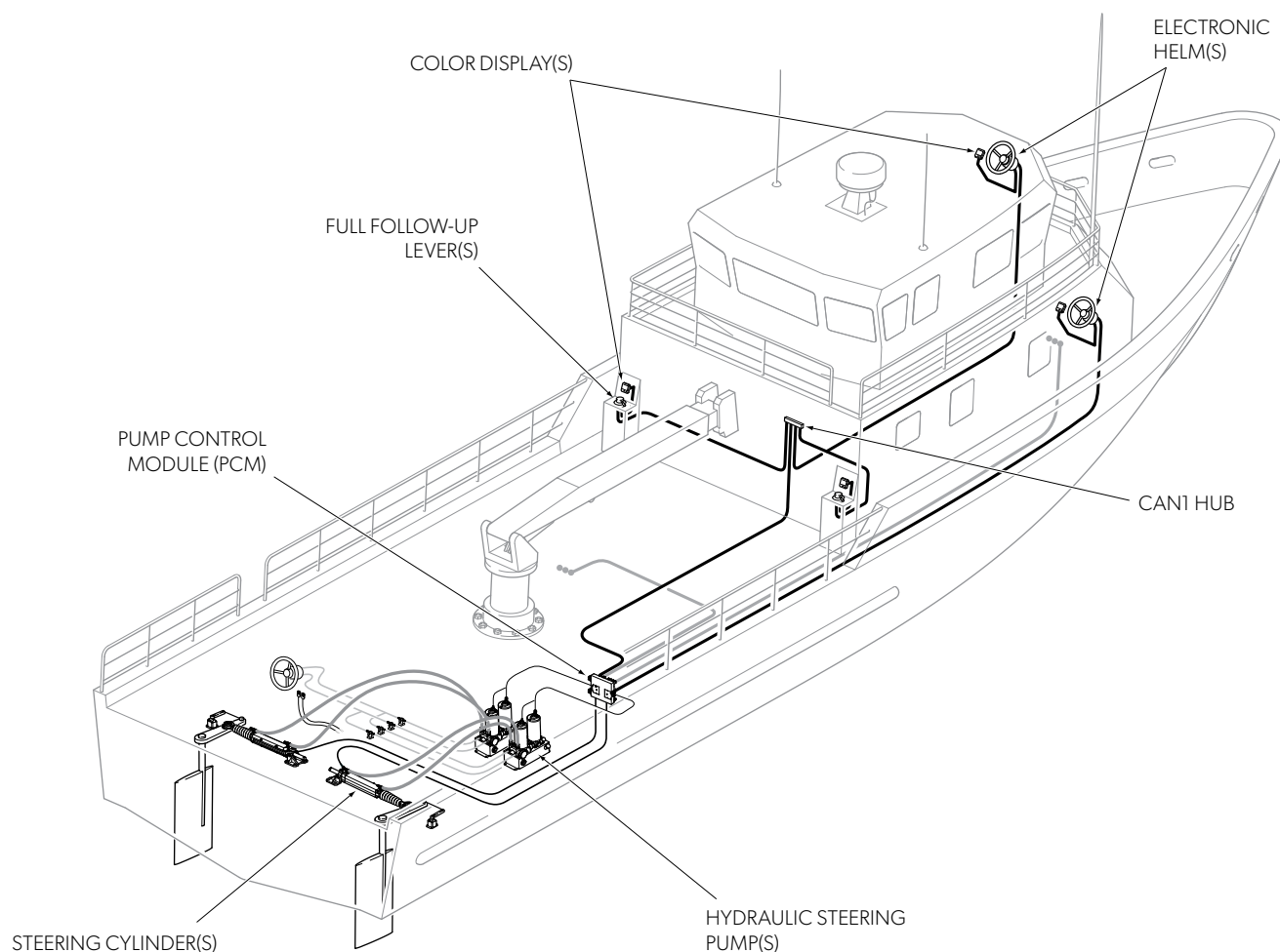
Figure 12-11. System components.
